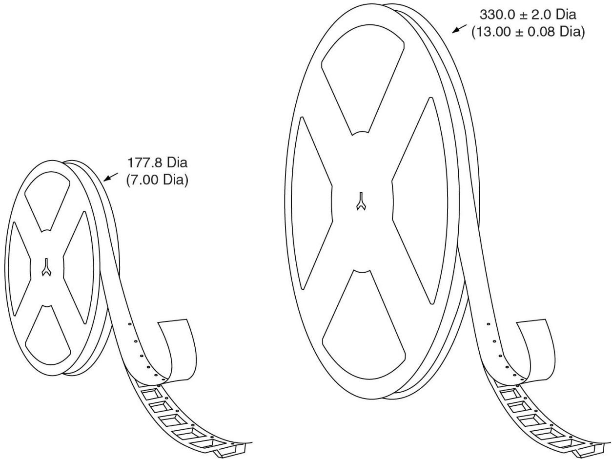
7 inch reel
